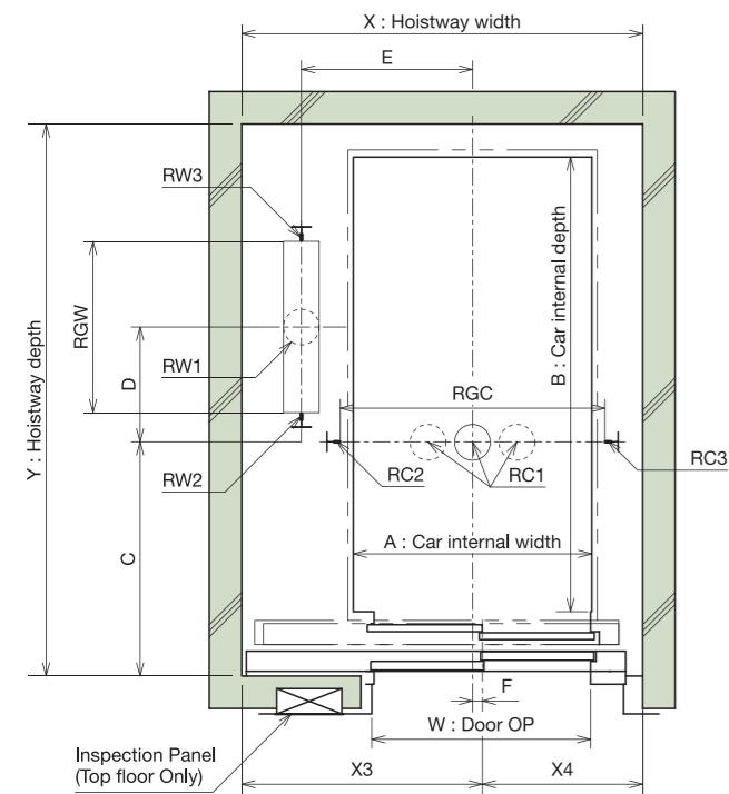
Hoistway dimension and Pit reaction loading
